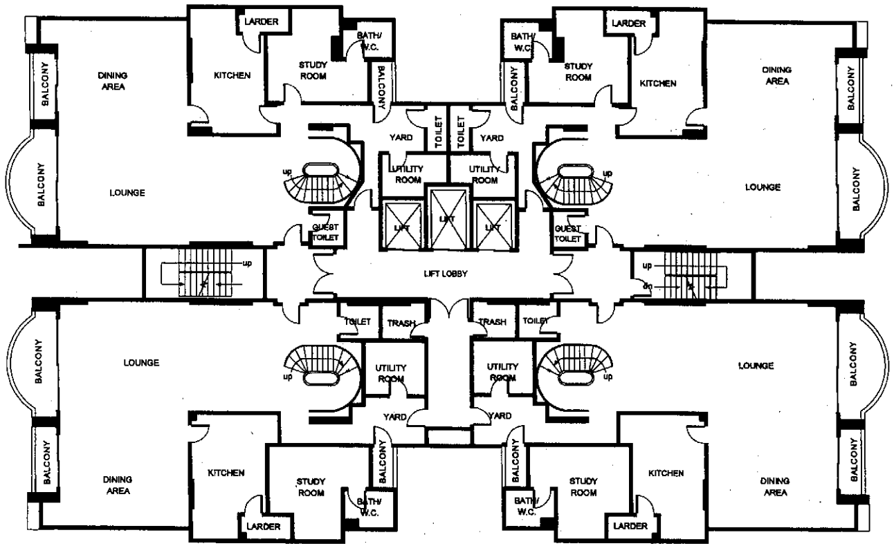
20TH FLOOR TO LOWER PENTHOUSE
